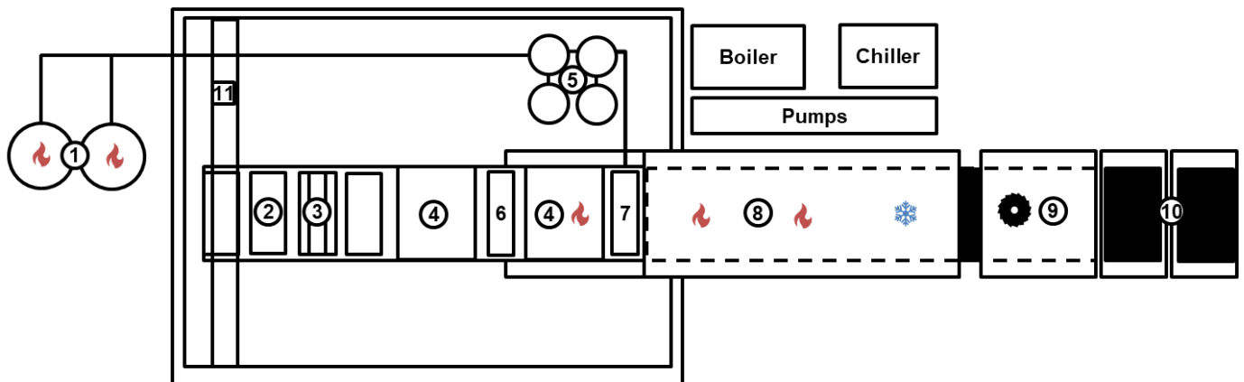
SIDE VIEW
